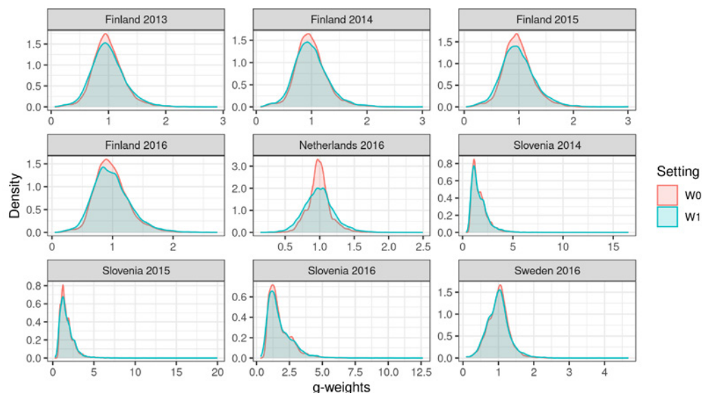
Figure 10.4: Density plots for calibration factors (g-weights)
